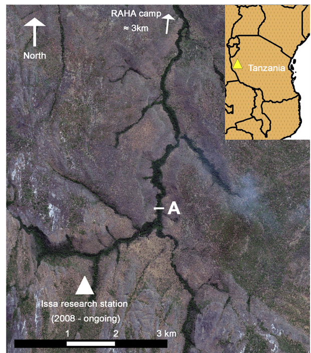
Figure 2. Central portion of Issa study area, Ugalla. The area shown is approximately 42 km 2 (cf. Gombe National Park ≈ 36 km 2 ); it is about half the area currently monitored on a regular basis. Width of the riverine evergreen forest strip at 'A' is ≈ 120 m.
