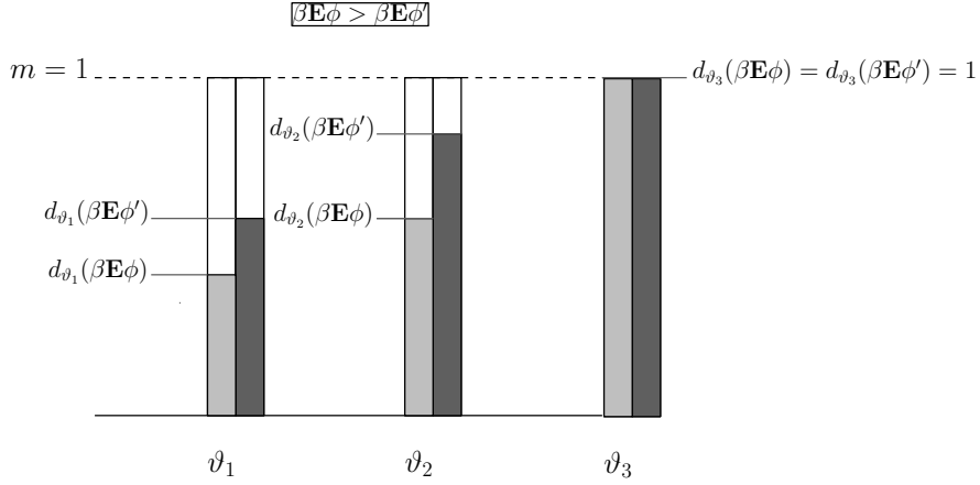
Figure 1: Money spent in decentralized market
