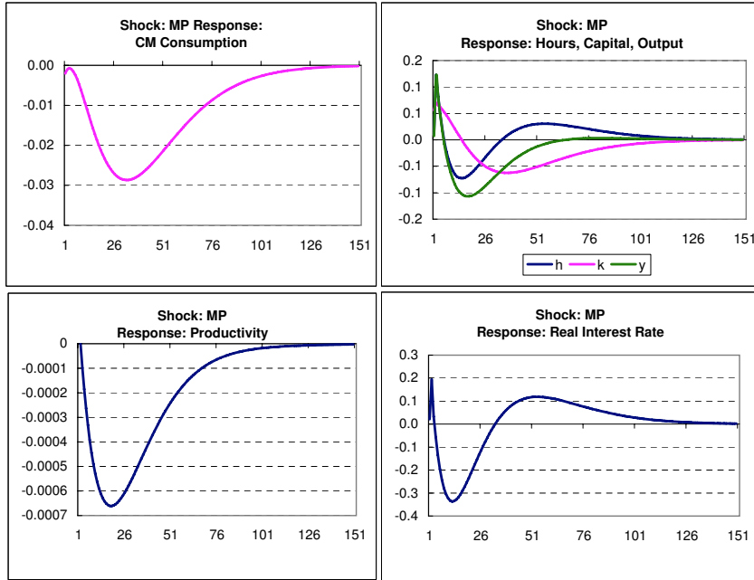
Figure 3: Real Variables' Impulse Responses to a Monetary Policy Shock, % of Steady State
