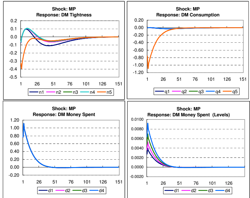
Figure 2: Decentralized Market Impulse Responses to a Monetary Policy Shock, % of Steady State
